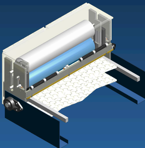
2RSCC-4IIA Top Side Cleaner
